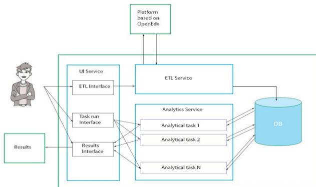
Fig. 1. Architecture of the application
