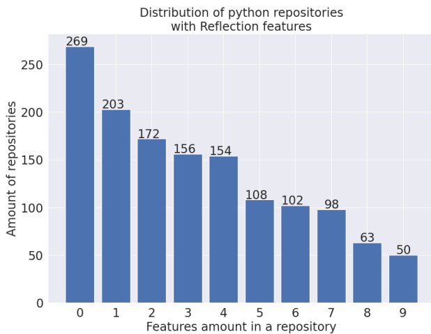
Fig. 10. Reflective code features in Python repositories
