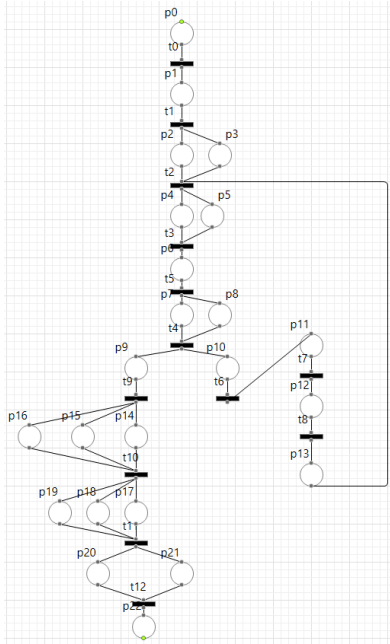
Figure 3. Logistic process "Ship boarding in the port" (temporary Petri nets)
