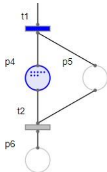
Figure 4. The result of the simulation experiment - a transition that cannot be performed is identified.
